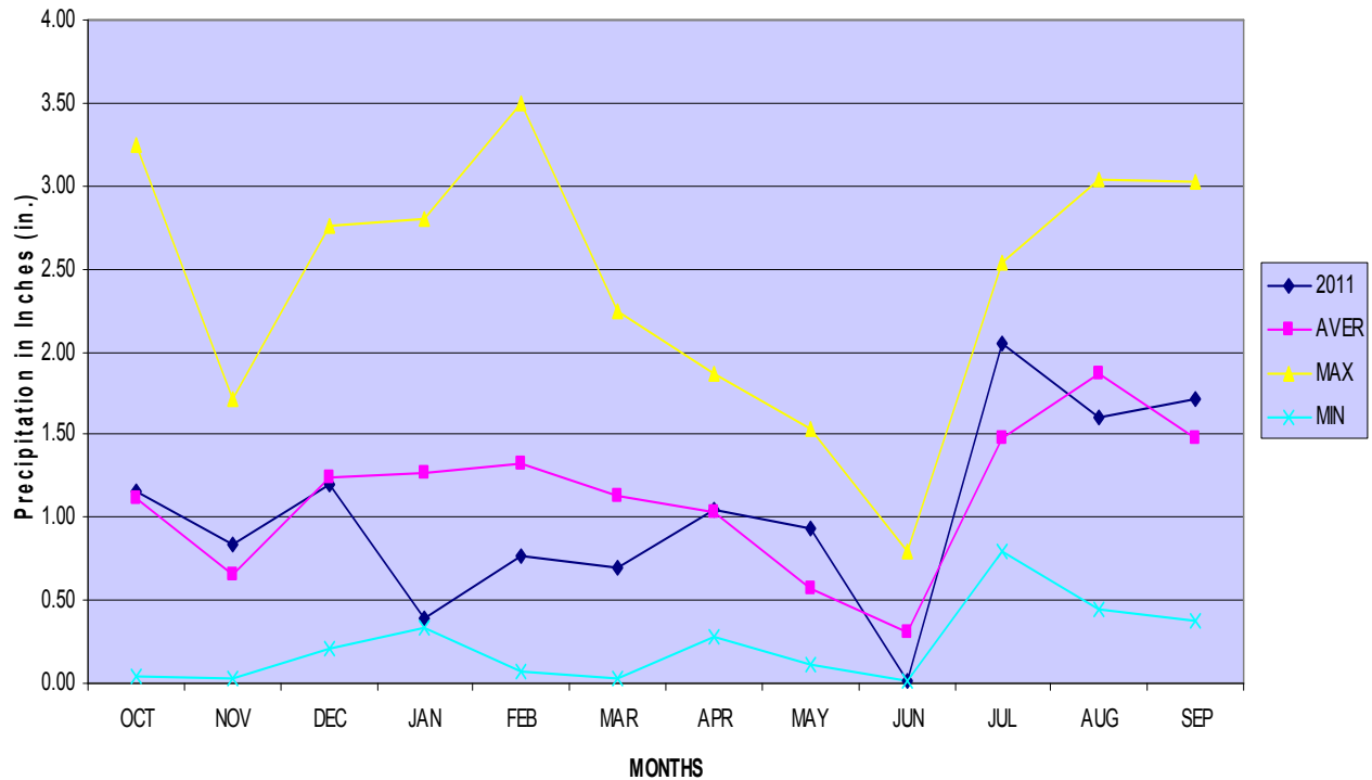
Average Precipitation for Chinle Agency (September 2011)
