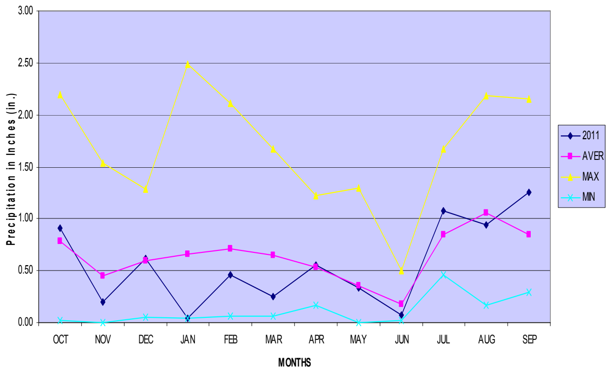
Average Precipitation for Western Agency (September 2011)
