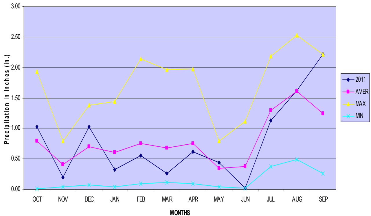
Average Precipitation for Eastern Agency (September 2011)
