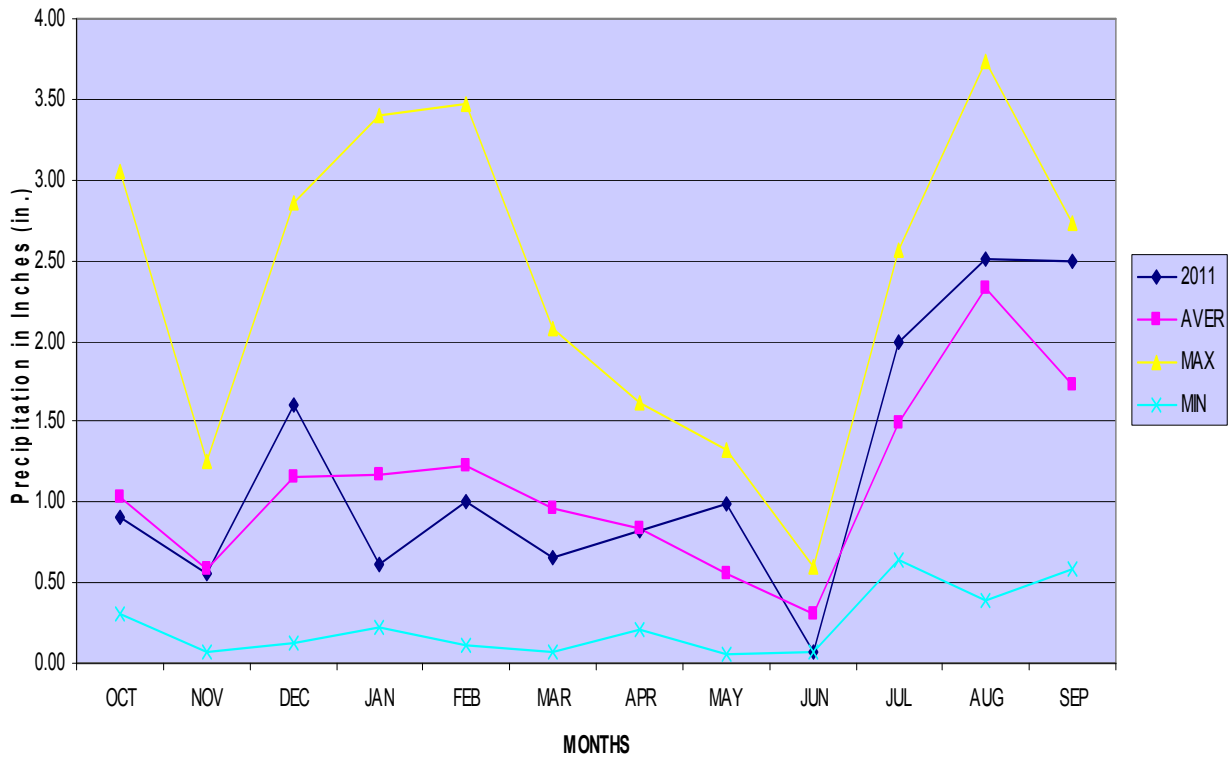
Average Precipitation for Fort Defiance Agency (September 2011)
