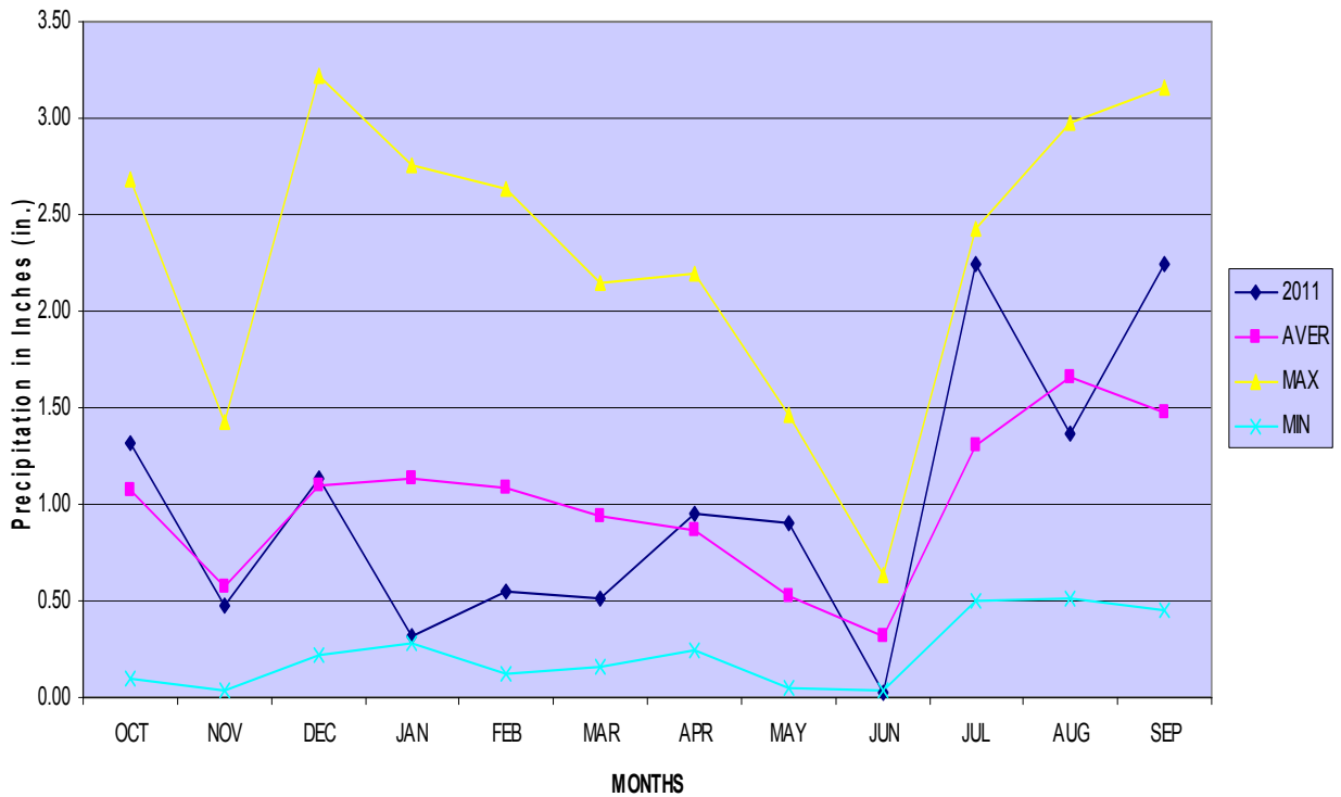
Average Precipitation for Shiprock Agency (September 2011)
