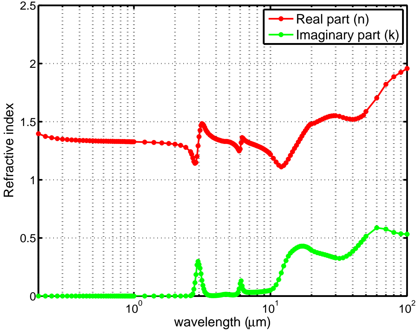
Refractive index of water, Hale & Querry (1973)
